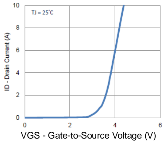
2. Transfer Characteristics
