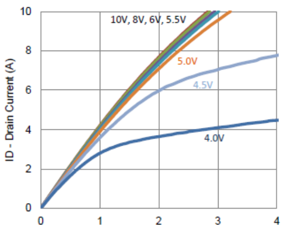
5. Output Characteristics
