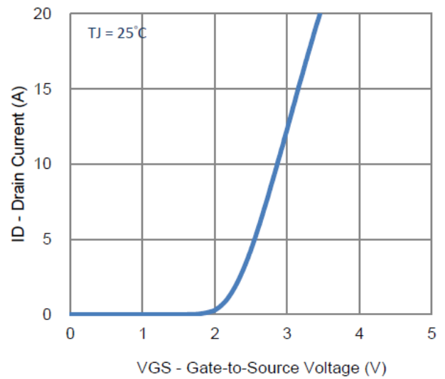
2. Transfer Characteristics
