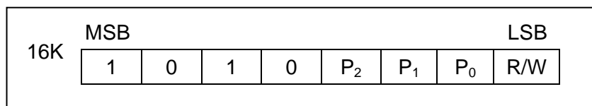
Figure 7 · Device Address
