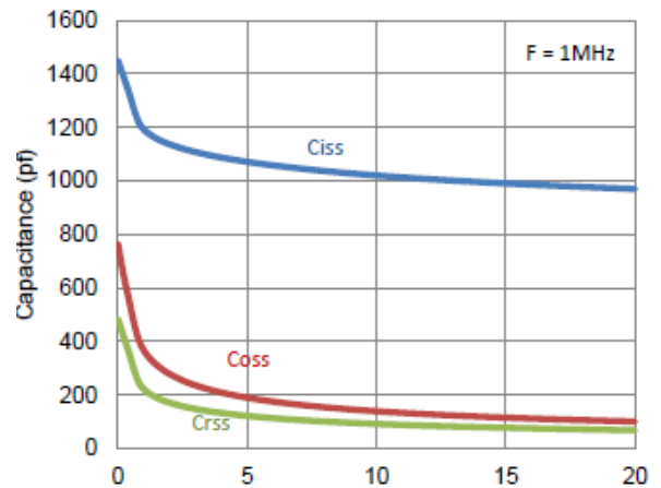
6. Capacitance
