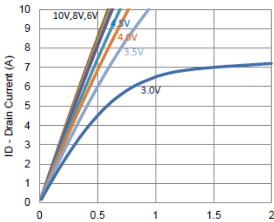
5. Output Characteristics
