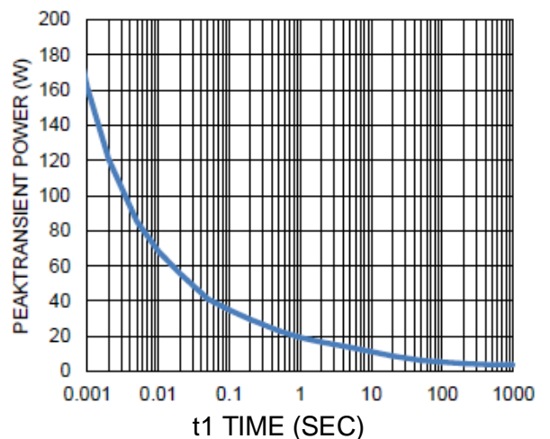
t1 TIME (SEC) 10. Single Pulse Maximum Power Dissipation
