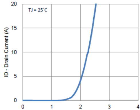
2. Transfer Characteristics
