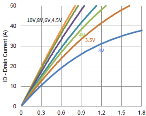
5. Output Characteristics
