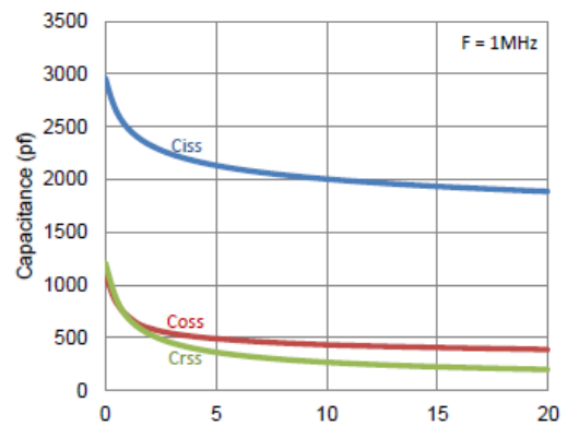
6. Capacitance
