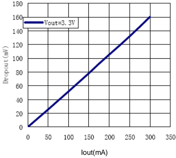
Dropout & Iout
