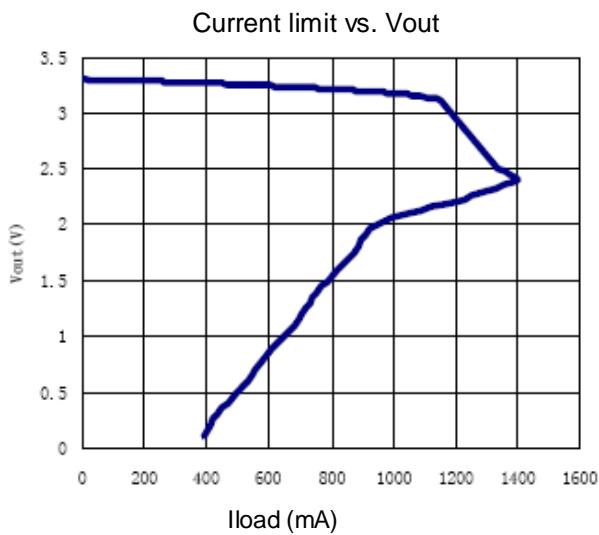
Output Voltage vs. Output Current (with output short protection)
