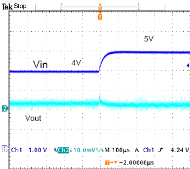
Line transient response Cin=Cout=1uF Iout=25mA Vout=3.3V
